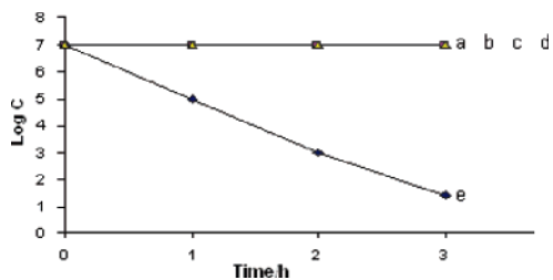
Figure 4. Temporal course of the E. coli inactivation ( 1 \times 10^7 , 30 mL) in aqueous dispersions containing 24 mg of catalysts (a) Ag/TiO 2 , (b) Ag/AgBr/TiO 2 , (c) apatite-covered TiO 2 , (d) TiO 2 /P-25, and (e) apatite-covered Ag/AgBr/TiO 2 under dark condition.
